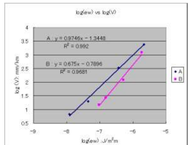
Wear Volume/1,000km VS Friction Energy
